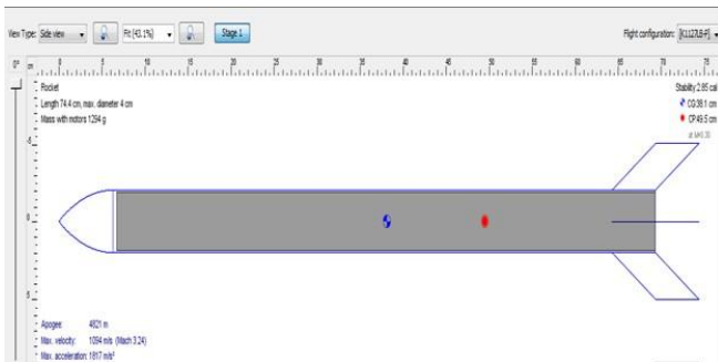
Figure:Twodimensionalfigureofmissile
