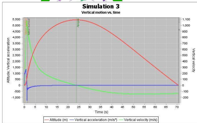
Figure:simulationofmissiles Simulation 1
