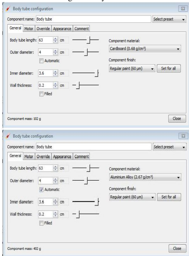
Figure: table of cylinder for missile with different materials Motor for missile:
